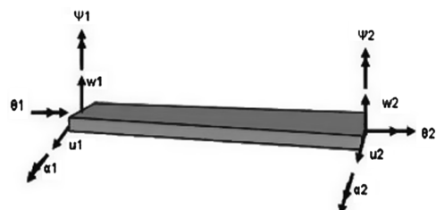
Fig. 3 Ten degree of freedom beam finite element BEMBLD.
